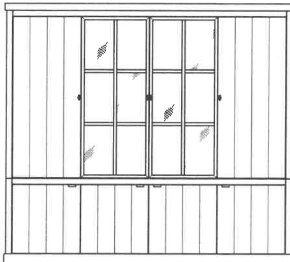
VITRINE 4DOORS (2DW + 2DM) 2410 x 480 x 2200(H)
