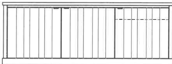
BUFFET 3 DOORS - 1 DRAWER 2380 x 480 x 885(H)
