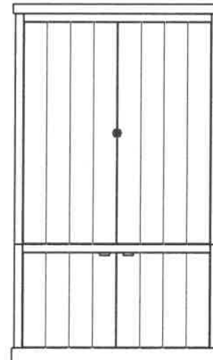
VITRINE 2 DOORS WOOD 1271 x 480 x 2200(H)
